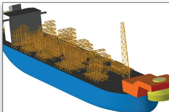
Data interchange with MOSES for FPSO topsides analysis.
