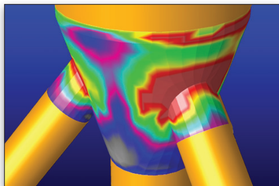
Parametric study for the fatigue design of a wind turbine transition piece.
